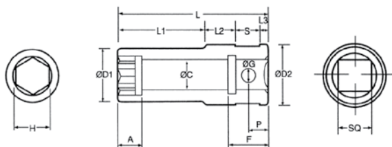
NUTRUNNER SOCKET TYPE A
